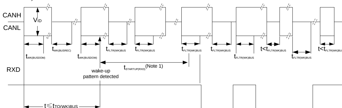
Figure 9-1. Wake-up Timing
