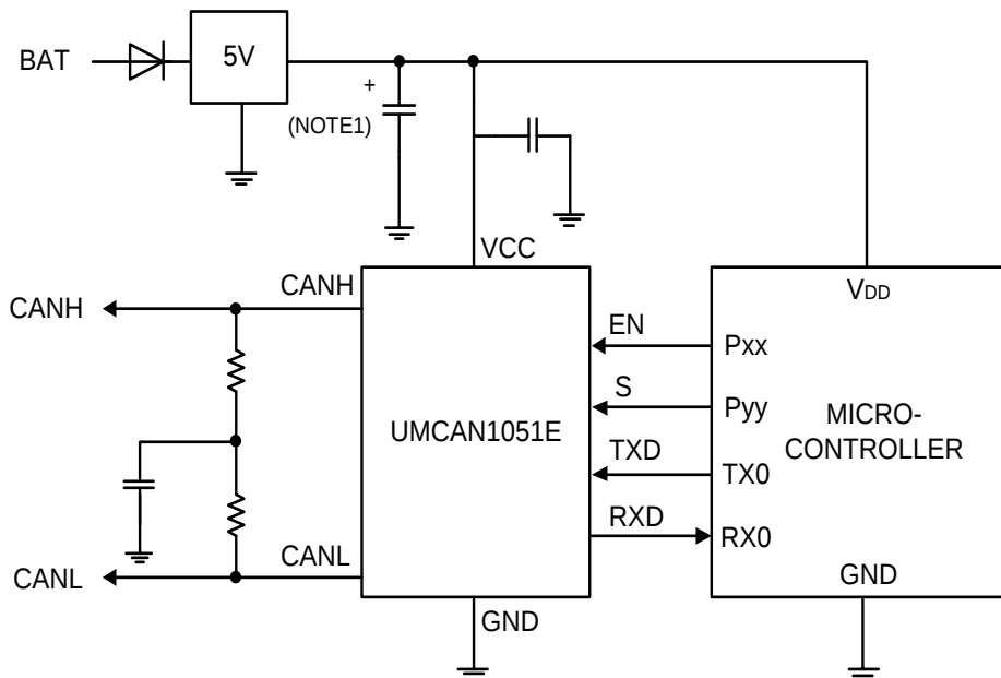
Figure 10-1. Typical application of the UMCAN1051E
