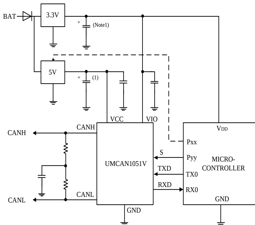
Figure 10-2. Typical application of the UMCAN1051V
