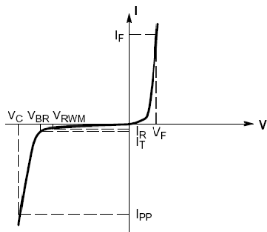
Uni-Directional TVS
