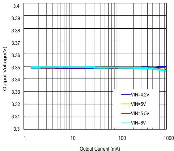
Output Voltage vs. Load Current V_{OUT}=3.3V , MODE=H
