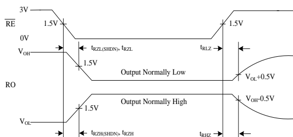
Figure 10. Receiver Enable and Disable Times
