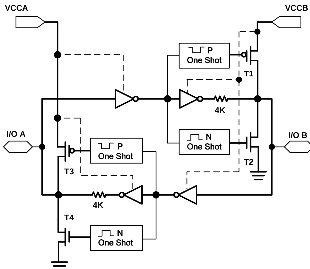
Figure 1 Block Diagram of UM3304/UM3304QS/UM3304QT/UM3304QA/UM3304UE I/O Cell
