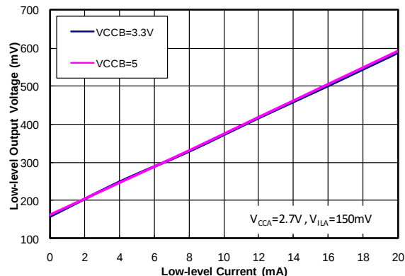
Low-level Output Voltage vs. Low-level Output Current
