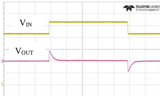
Line Transient Response
