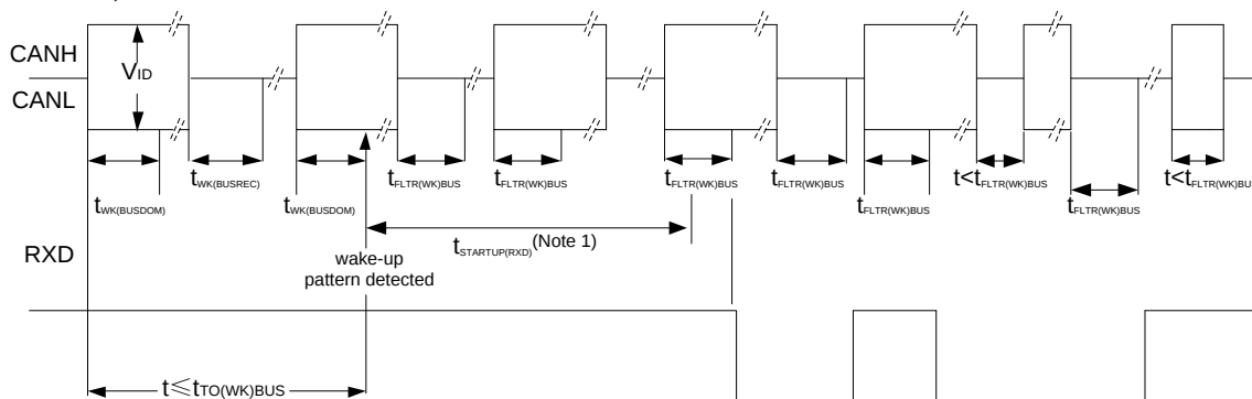
Figure 9-1. Wake-up Timing
