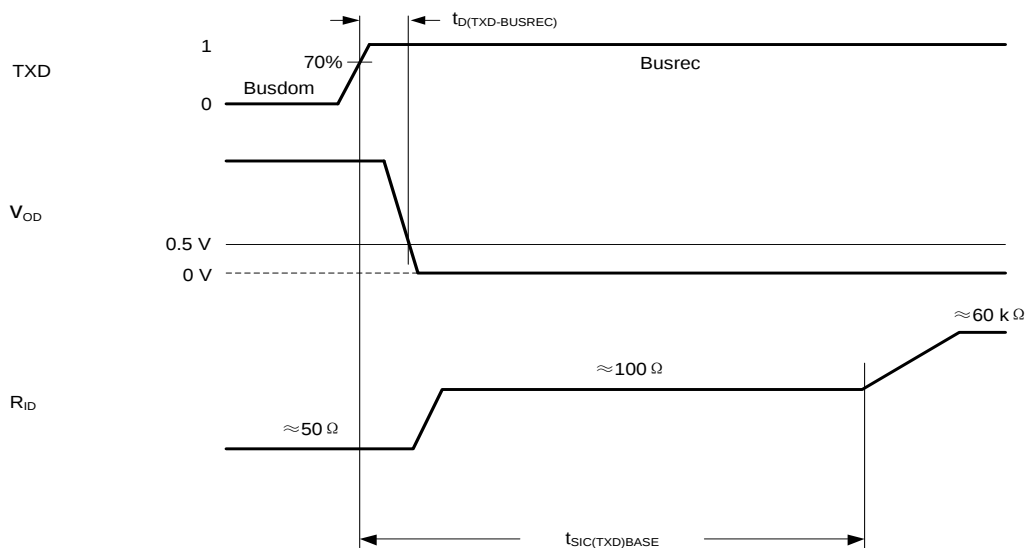
Figure 7-5. UMCAN1472 transmitter impedance and timing diagram for dominant-to-passive recessive transition
