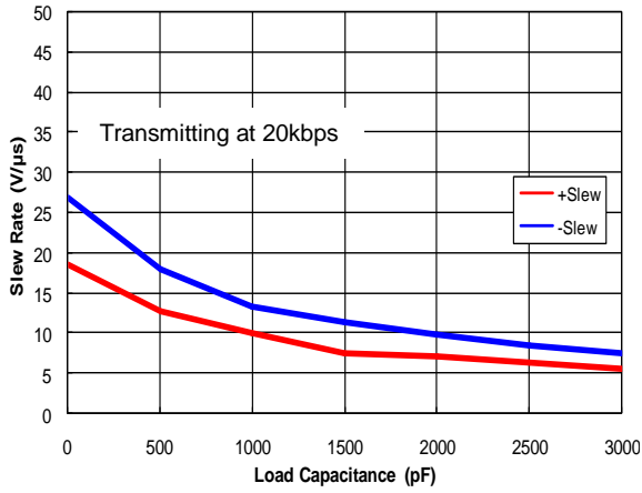
Slew Rate vs. Load Capacitance
