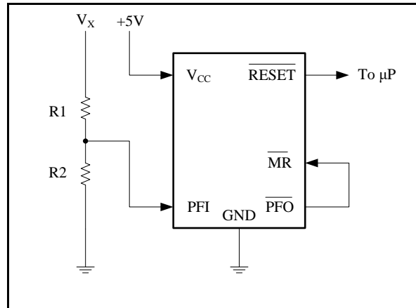
Figure 10. Monitoring an Additional Supply V_x
