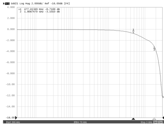
Differential Bandwidth
