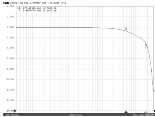
Differential Bandwidth
