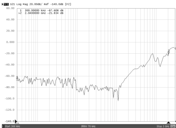
Crosstalk
