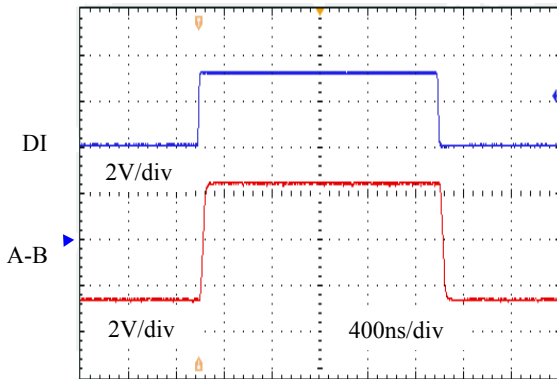
Transmitter Propagation Delay R_L=54\Omega , C_L=100pF
