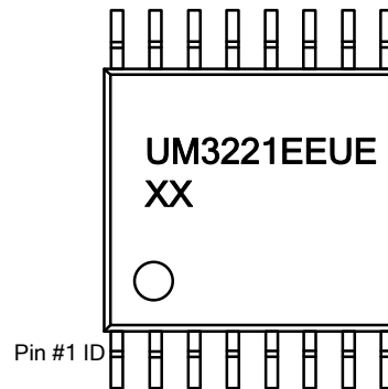
XX: Week Code UM3221EEUE TSSOP16
