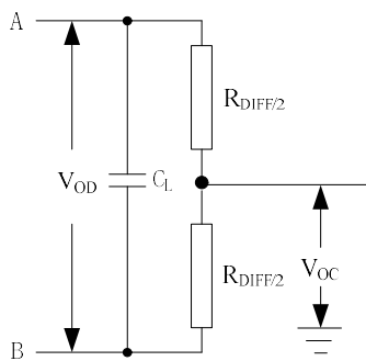
Figure 1. Driver DC Test Load
