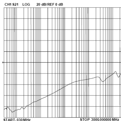
Analog Crosstalk
